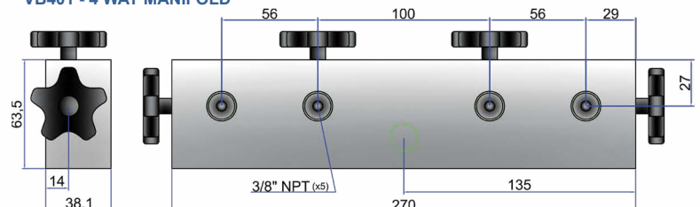
VB401 - 4 WAY MANIFOLD
