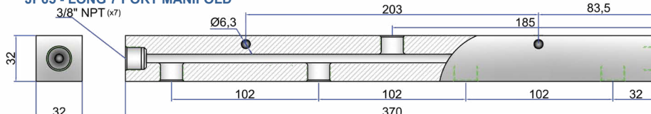
JP65 - LONG 7 PORT MANIFOLD
