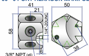
JP66 - 6 PORT HEXAGON MANIFOLD
